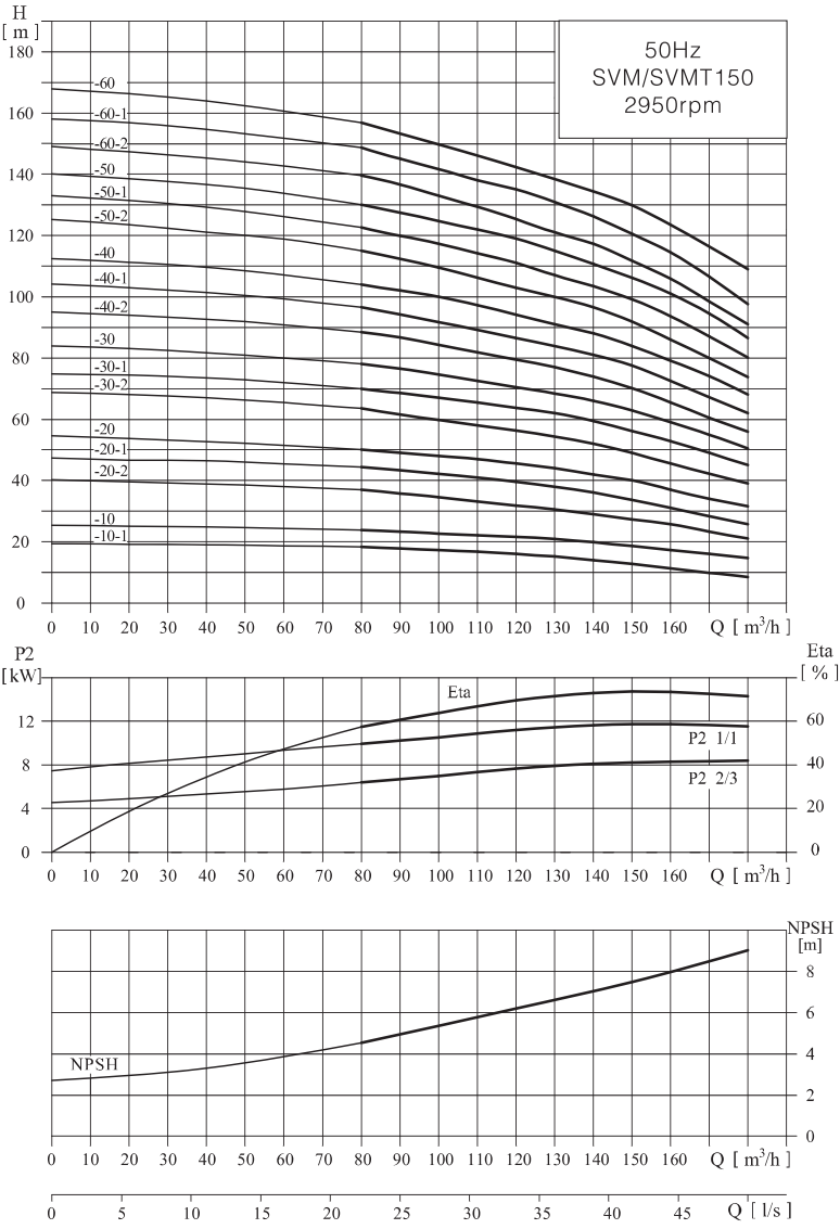
Performance cruve
