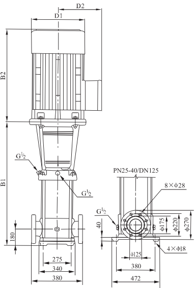
Installation dimensions and weight
