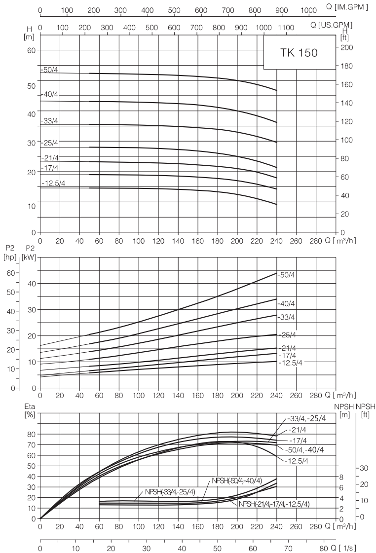
Performance cruve
