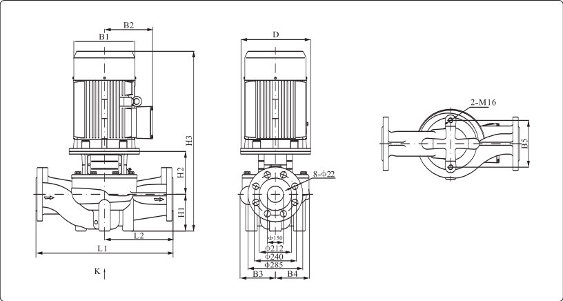
Installation dimensions and weight
